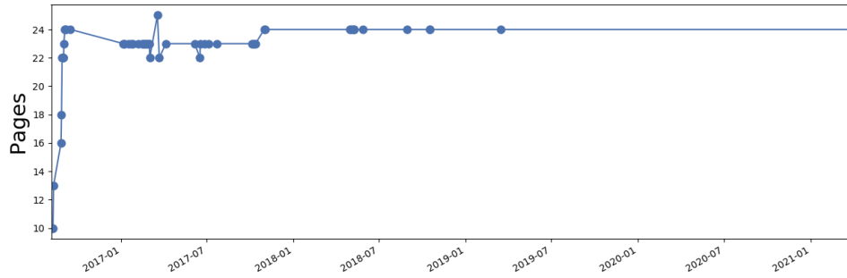
Figure 4: Page count over time.
