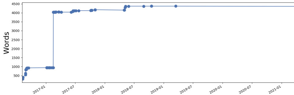
Figure 5: Word count over time.
