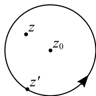
Figure 3.3: Region for Taylor Expansion
