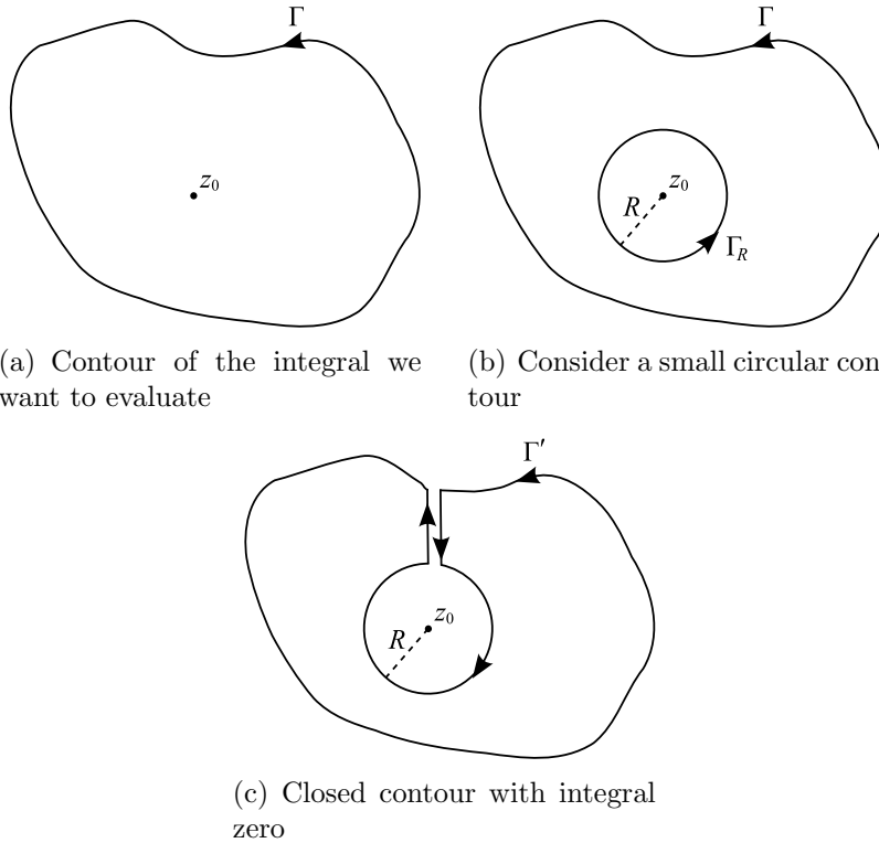
Figure 3.1: Demonstrating the Deformation Theorem
